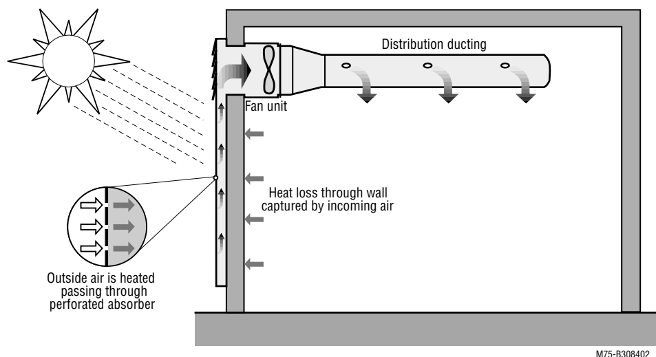
Figure 3. Transpired collector operation during the winter months.
